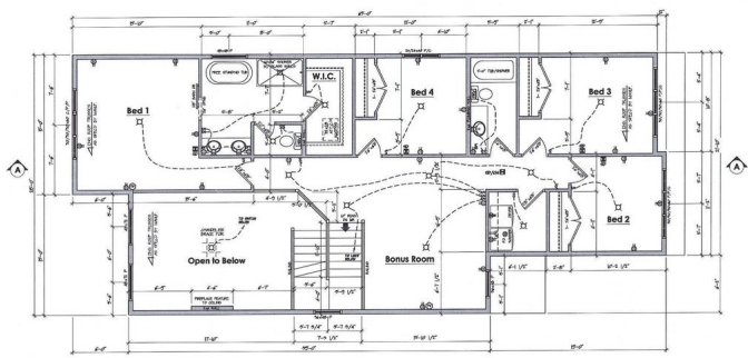
Second Floor Plan 1206 sq ft
